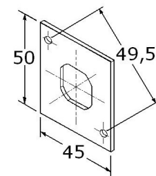
Mounting plate with holes 43.295
