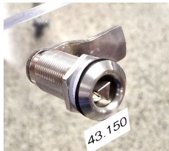
Cam latch #43.150 with hook cam #43.227 & Cam 43.112
