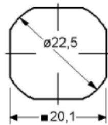
Diameter 22.5 mm
