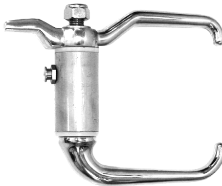
#44.941 | Extra heavy duty 316 stainless steel door dogging device with aluminum bushing 73 mm
