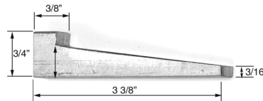
#44.943 Strike wedge weld on type for door dogging device
