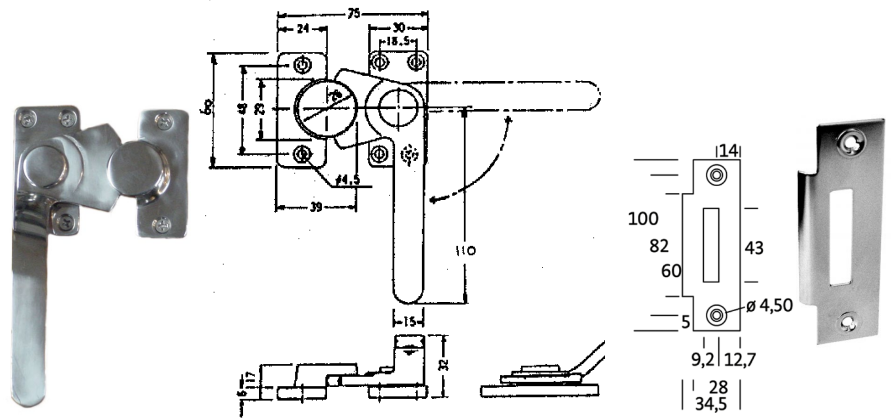
Left Hand Right Hand #44.221 304 stainless steel dogging device for hatches & doors. Strike 43.141 with lip #43.141 Strike with lip: 28 x 100 x 1.5 mm. Allows for angle mounting
