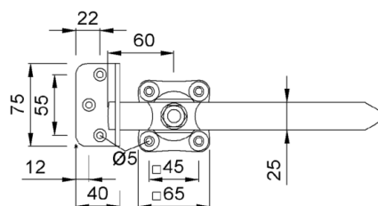
#44.130 Door toggle; single sided with angle strike plate. 304 stainless steel
