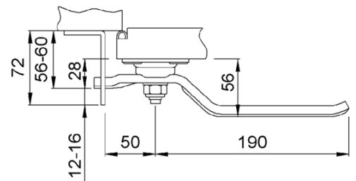
#44.130 Door toggle; single sided with angle strike plate. 304 stainless steel
