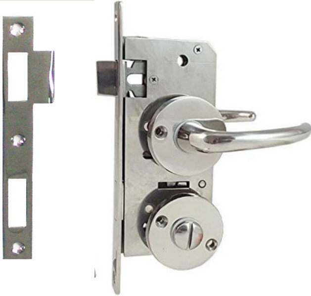
Set: # 16.350W Small Privacy lock; Stainless steel. 1 9/16" backset or 40 mm.
