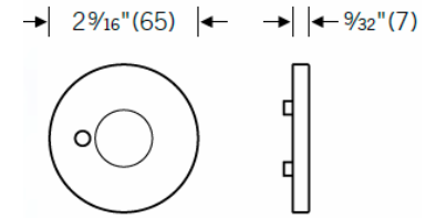
#12.179815 Rose for tubular privacy latch 65 mm diameter
