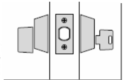
12.238134 #12.23834 Dead Bolt 2 3/4" backset with strike box for key/key or key/ thumb-turn 12.238138 #12.23838 Dead bolt 2 3/8" backset with strike box; for key/key or key/ thumb-turn
