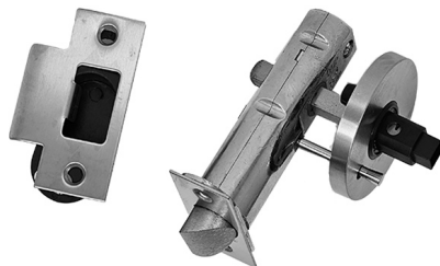
Privacy latch - Showing options with 55 mm diameter Roses
