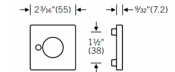
#12.170315 Square rose for tubular privacy latch; 55 x 55 mm
