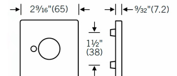
#12.170515 Square rose for tubular latch 65 x 65 mm
