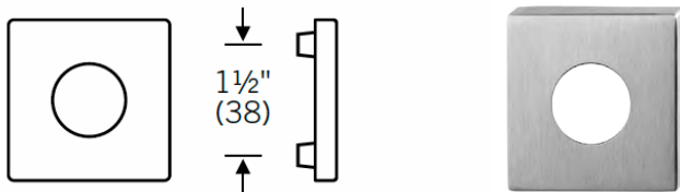
Stainless steel rose square, pair #12.1703 Screws invisible 55 x 55 mm or 2 3/16 inch. Clip on style with inner rose.
