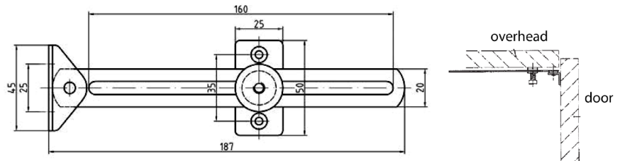
Door stay #33.654.266 light duty, 160 mm travel.
