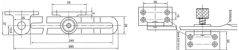
#33.065A.508 Door stay heavy duty with brake and endstop; With Angle Bracket 235 mm travel, ~ 9 1/4"
