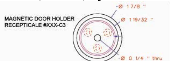
#34.MDH in polished chrome Magnetic door holder Wall or floor or ceiling mounted; For medium weight doors distance: 75.5 mm - 3"high . Brass base material, except for magnet Cup in receiver part galvanized steel.
