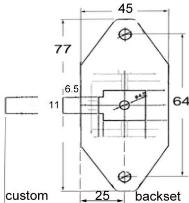
#25.5275 SET with S / S push button set; 25 mm backset Drill hole 25 mm diameter for ring
