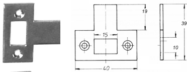
Strike plate for 3/4 inch doors
