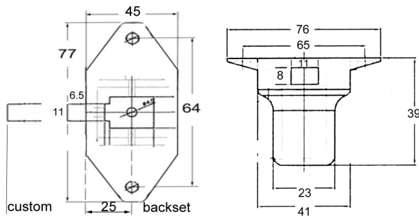
Dimensions mechanism in mm.
