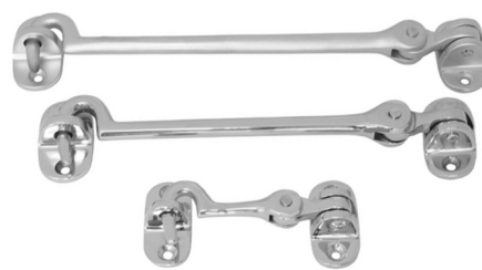
Ajar Hooks: Hook length (A) : 2", 3", 4", 5", 5 7/8", 6 7/8", 7 7/8" (add : 1" for door to wall length)
