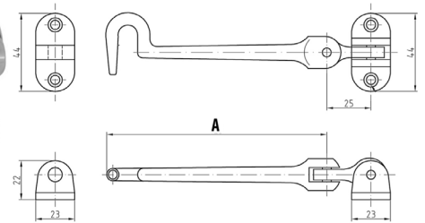
Ajar Hooks: Hook length (A) : 2", 3", 4", 5", 5 7/8", 6 7/8", 7 7/8" (add : 1" for door to wall length)
