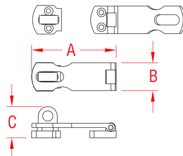
#33.3853.208 The Safety Hasp is precision cast and easily installed using #8 fasteners. A= 3 inch B= 1 inch C= 1.16 inch
