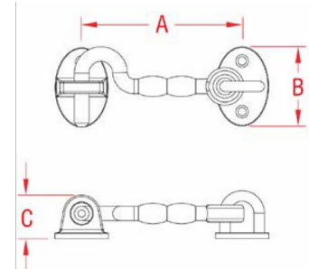
33.3851.208 Ajar Hook Length 3 inch. Stainless steel 33.3852.208 Ajar Hook Length 4 inch. Stainless steel A= 3 and 4 inch B= 1.48 inch C= 0.82 inch
