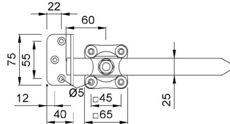
right hand setup depicted with bracket mounted outward
