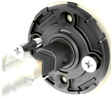
#12.110N.308 Spring loaded rose 55 mm diameter for use with matching levers and 8x8 mm spindle
