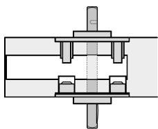
Rose #12.42311 tubular dummy plate with face plate (not shown) use with any lever with 18 mm diameter collar Drill hole 18 mm diameter for 8 x 8 mm spindle
