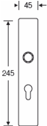
#12.1410 escutcheon Stainless steel clip on model
