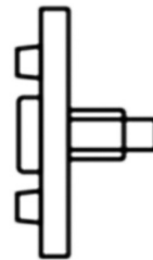
#12.110N.308 Spring loaded rose 55 mm diameter for use with matching levers and 8x8 mm spindle
