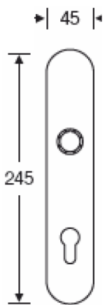
#12.222 Escutcheon stainless steel clip on model
