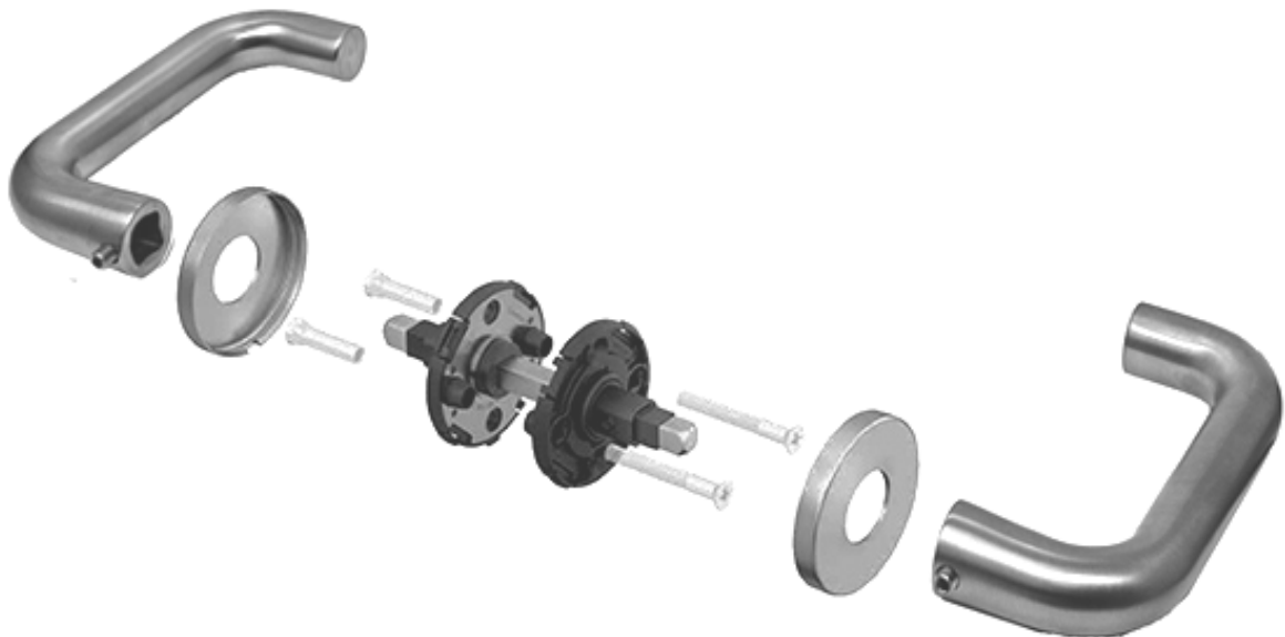
Exploded view of sample of assembly spring loaded roses #12.110N.308 with our matching levers with 8x8 mm stainless steel spindle. Depicted here with lever #12.045
