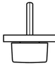
#12.329.508 thumb-turn / indicator with 55 mm roses. Polished stainless steel available with 8x8 mm spindle or 7x7 mm spindle
