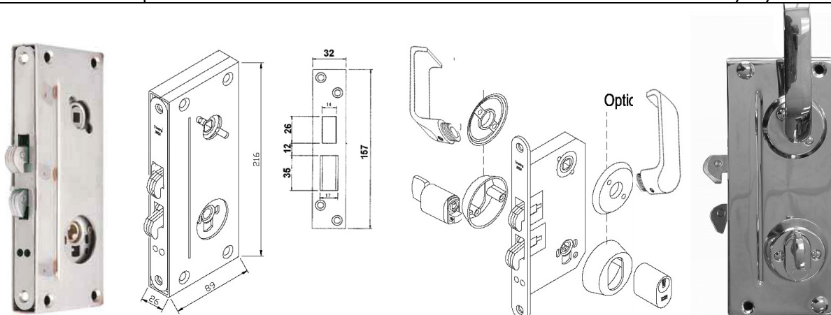
#11.SBET01; Complete SET Rim Mounted Sliding Box Lock. Lock and Box Stainless steel. Roses and Keyway Chrome Plated Brass.
