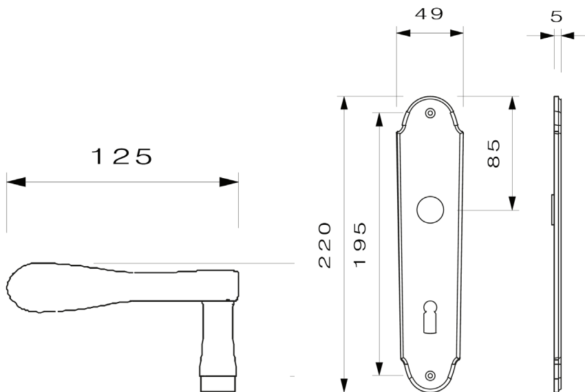
Lever Belvedere #13.J908 with Escutcheon 13.J988
